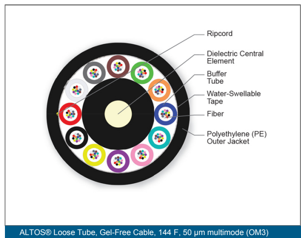
ALTOS® Loose Tube, Gel-Free Cable, 144 F, 50 µm multimode (OM3)
